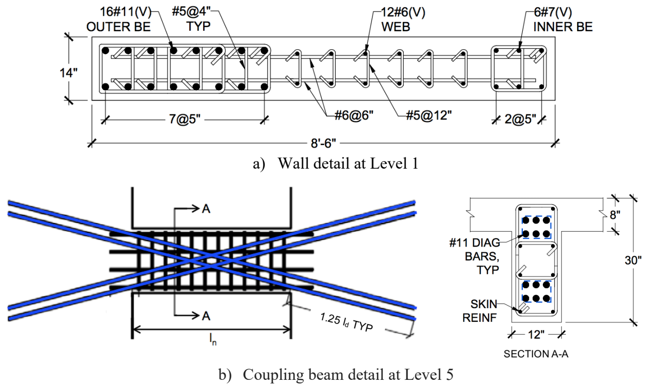
Figure 2.8: Archetype 8H-DR-3.0 Wall and Coupling Beam Details
