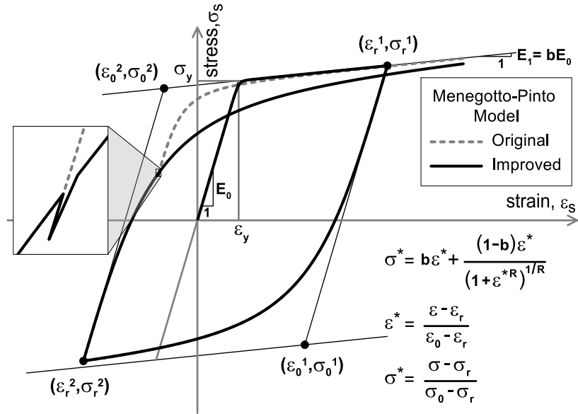
Figure 3.6: Material model for steel (Koložvari et al., 2017)
