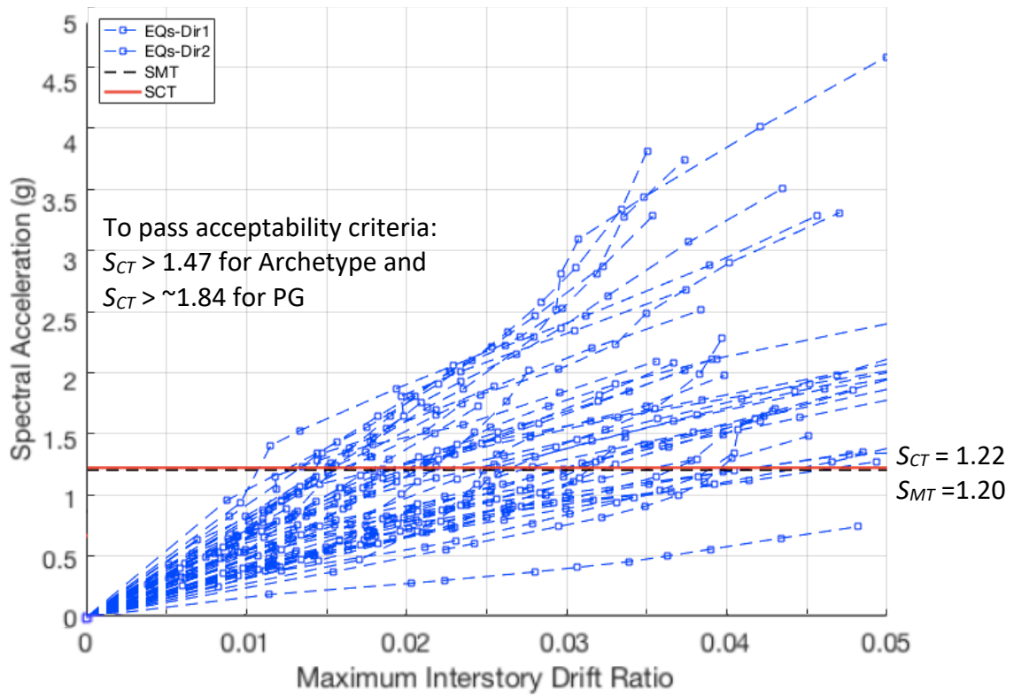
Figure 5.2: CMR Plot for Preliminary Archetype 8H-DR-3.0 designed per ACI 318-14
