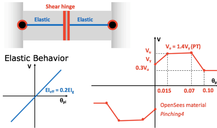
a) Typical modeling approach for coupling beams
