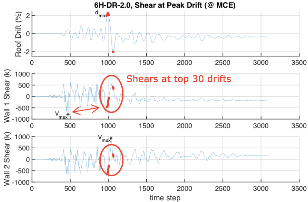
Figure 5.15: Shear at Peak Drift for Archetype 6H-DR-2.0
