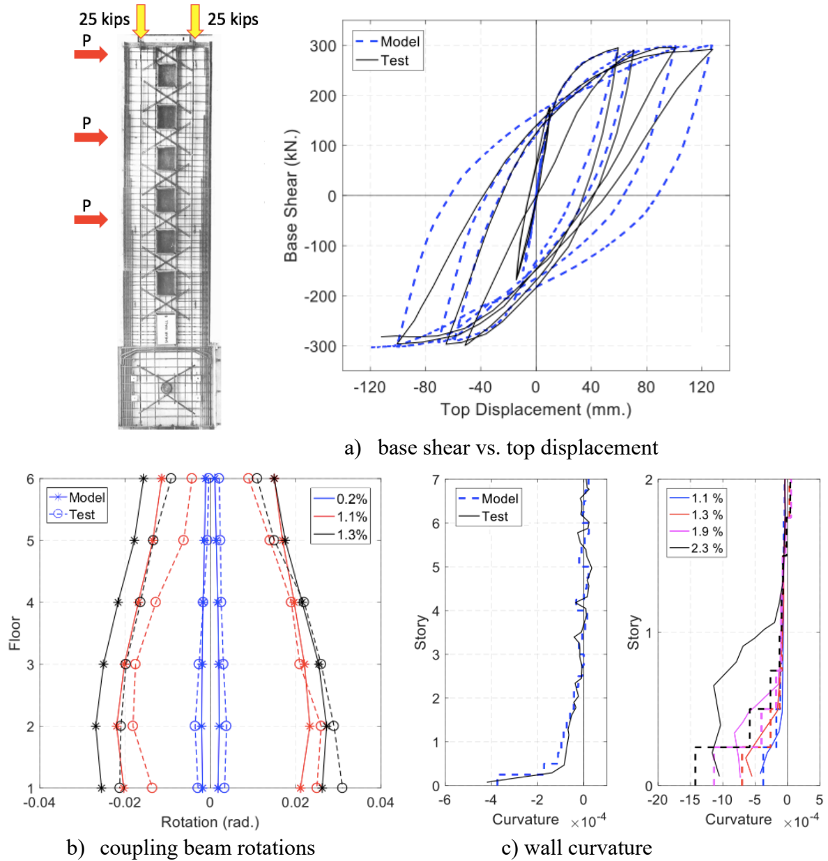
Figure 3.20: Model validation using Santhakumar test specimen (Kolozvari et al., 2018): a) base shear vs. top displacement, b) coupling beam rotations, c) wall curvature
