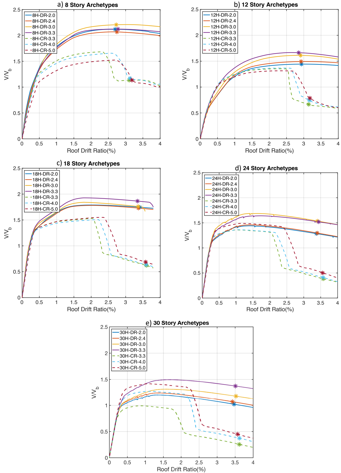
Figure 5.4: Pushover Curves for various Archetypes
