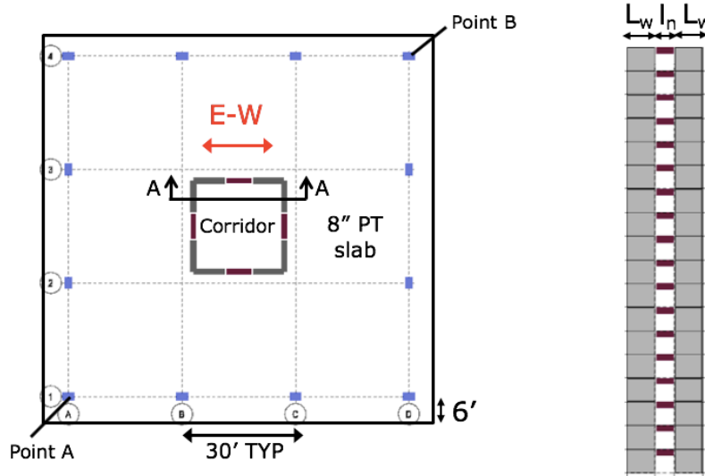
Figure 2.15: 18-Story Archetype
