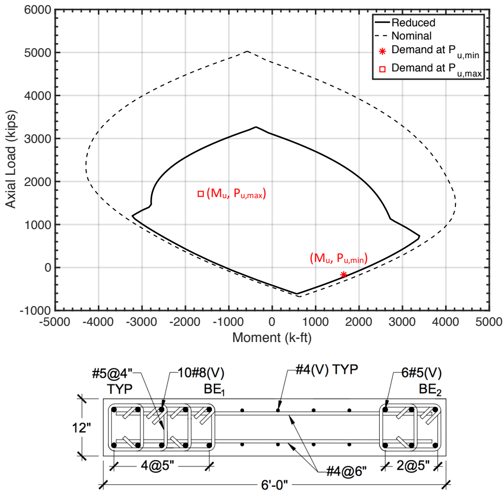
Figure 6.2: Archetype 12H-DR-3.0-D min Level 1 Wall P - M Interaction
