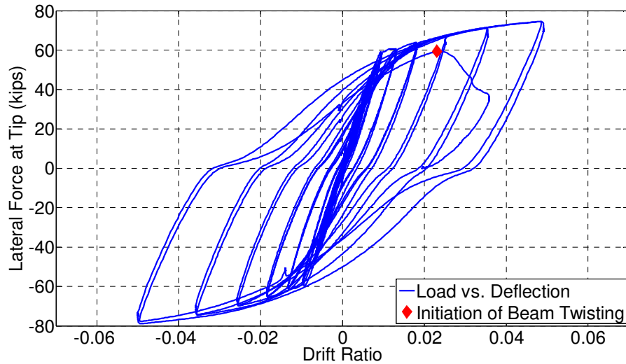
Figure 3.4.1: Lateral Force vs. Deformation – SBH60
