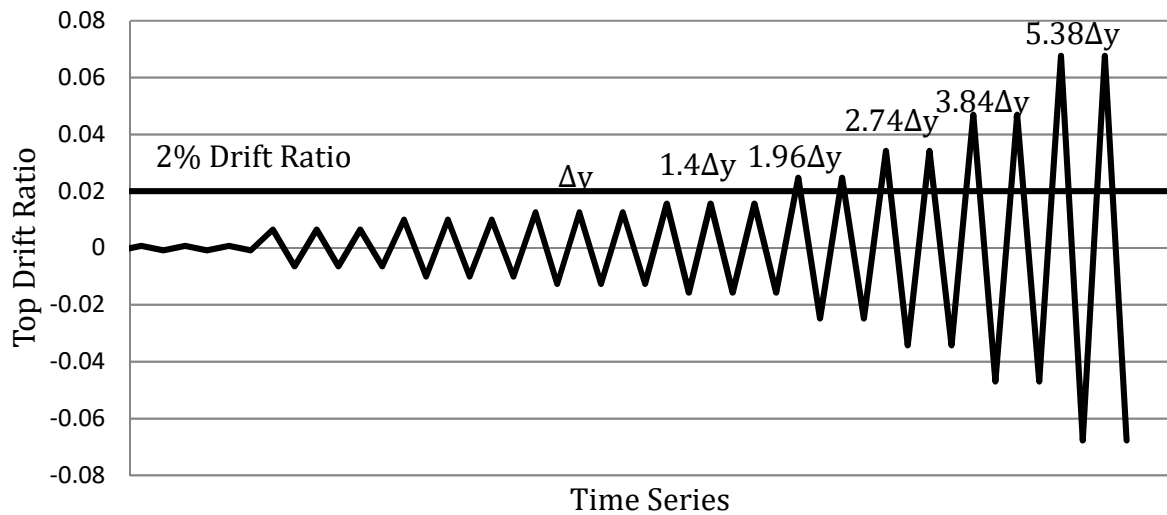
Figure 2.2.5: Loading History
