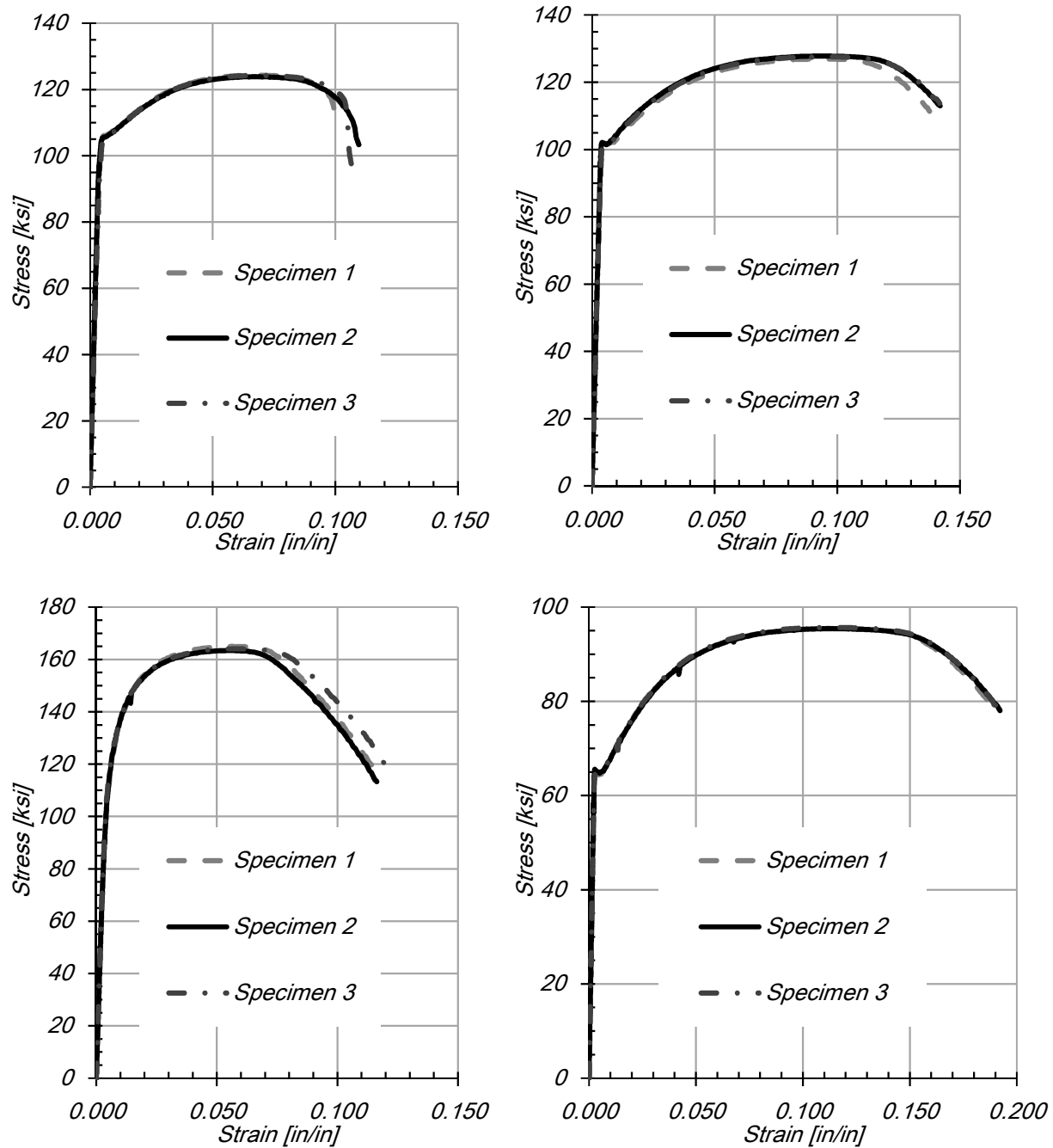
Figure A-9: Tension Stress-Strain relationship of Steel Coupon Tests: Top Left: No. 8 Bars Used in Beam SBL100; Top Right: No. 8 Bars Used in Beam SBH100; Bottom Left: No. 8 Bars Used in Beam SBM100; Bottom Right: No. 9 Bars Used in Beam SBH60
