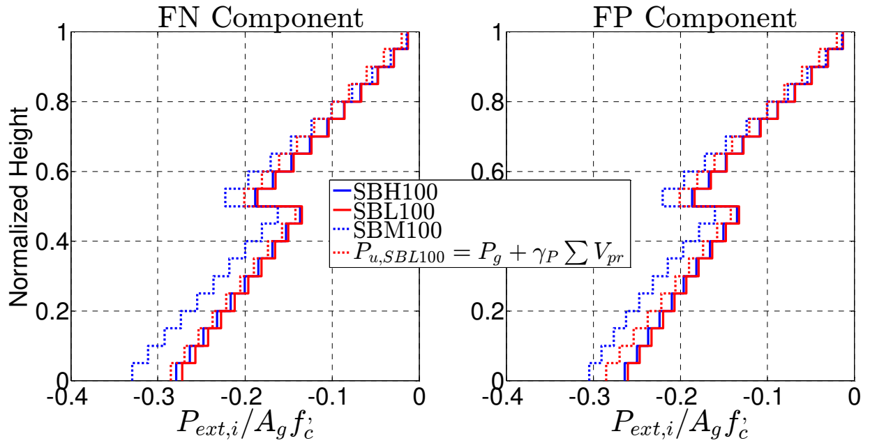
Figure 6.7.11: Exterior Column Compression in Frames SBH100, SBL100, and SBM100
