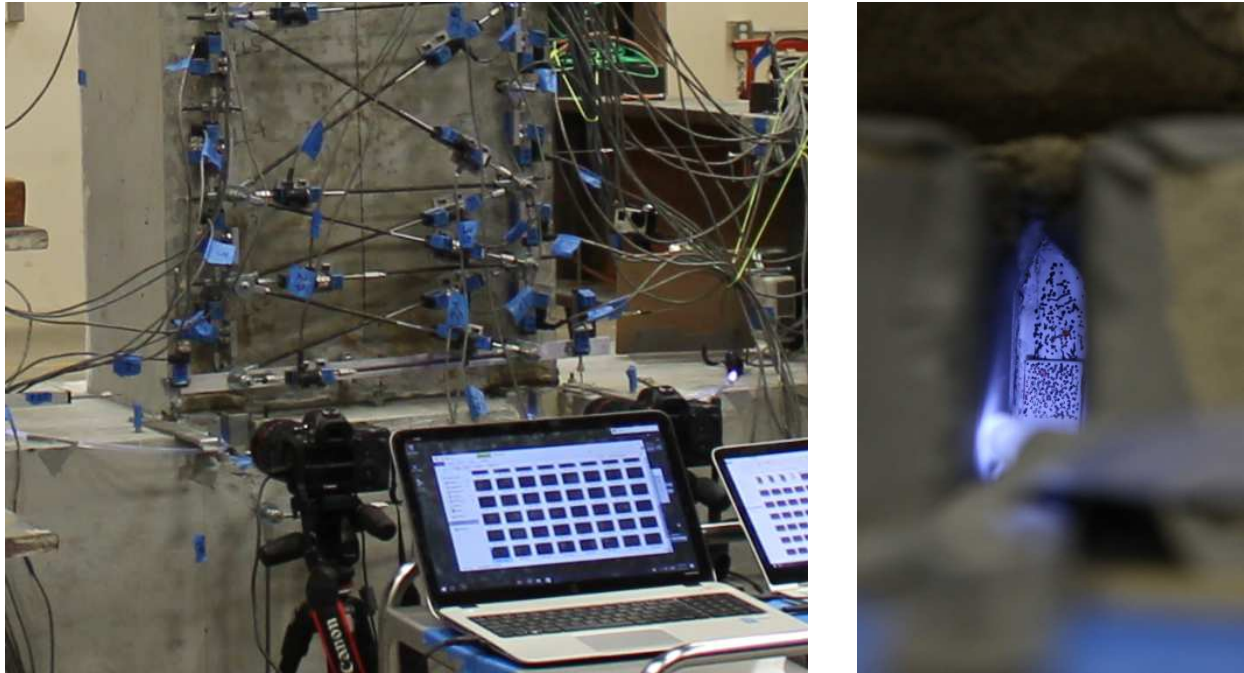
Figure A-22: General Instrumentation for Measuring Slip by Digital Image Correlation (DIC)
