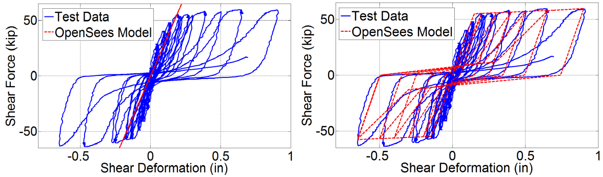
Figure 5.1.12: Shear Behavior – Left: Linear Elastic – Right: Ibarra-Medina-Krawinkler Model
