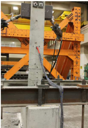
Figure 3.3.1: Failure Mechanism of SBH60 by Twisting of Beam (Global Instability)
