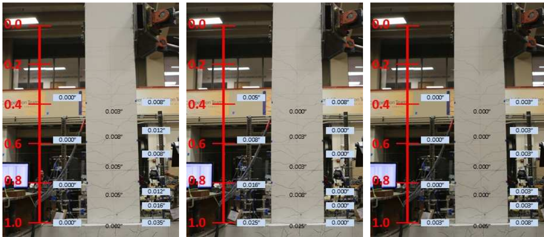
Figure C-4: Measured Crack Widths at Drift Ratio of 0.9% – Specimen SBH60
