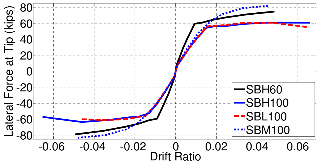
Figure 3.4.5: Force-Deformation Envelopes
