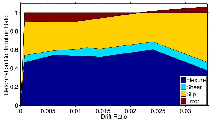
Figure 3.5.3: Deformation Components – SBL100
