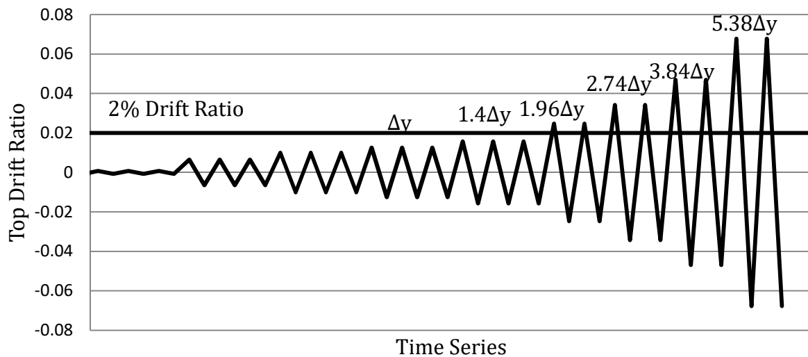
Figure A-26: Loading History
