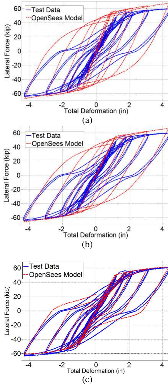
Figure 5.1.19: Overall Response of OpenSees Models. (a): Inelastic Flexure and Elastic Shear; (b): Inelastic Flexure, Elastic Shear and Slip; (c): Inelastic Flexure, Shear by Modified Ibarra-Medina-Krawinkler Model, and Slip by Fiber Section with Bond-Slip Steel Model by Zhao and Sritharan
