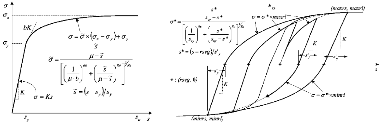
Figure 5.1.14: BondSPI Hysteretic Model Proposed by Zhao and Shritharan (2007)
