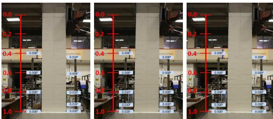
Figure C-16: Measured Crack Widths at Drift Ratio of 0.6% – Specimen SBL100
