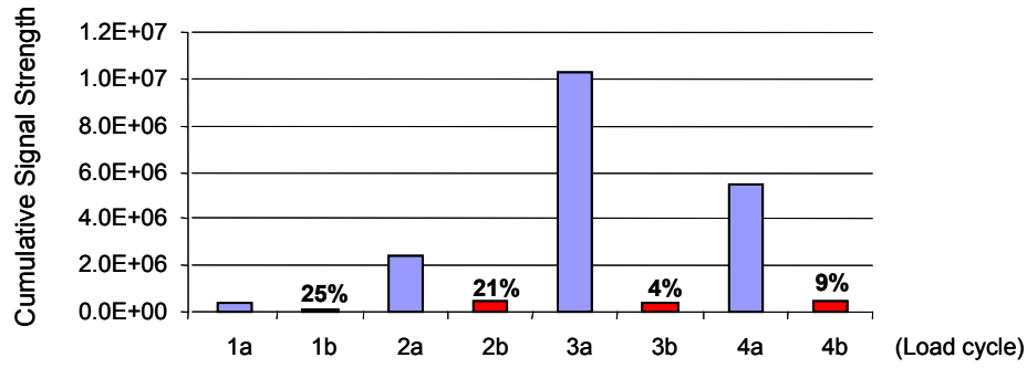
Figure 5.3a: Cumulative Signal Strength Ratio Results (with Simulated Shear Collar)
