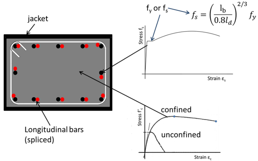
Figure 3-9 Assumed uniaxial stress-strain models
