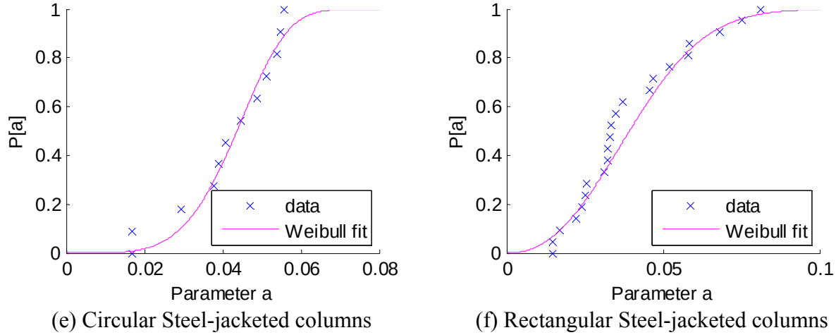
Figure 4-4 Empirical data cdf with the final distributions
